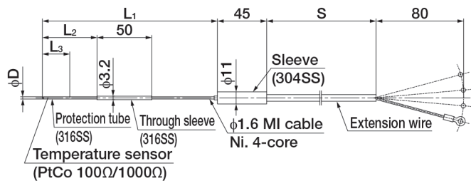
Fig 2. Sheath type
